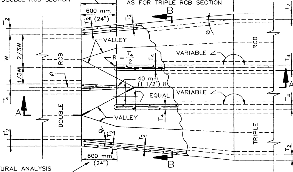
SECTIONAL PLAN
